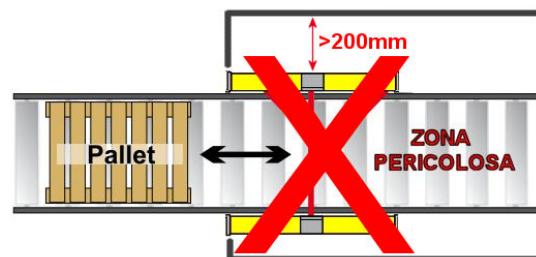
Mechanical protection incorrect
