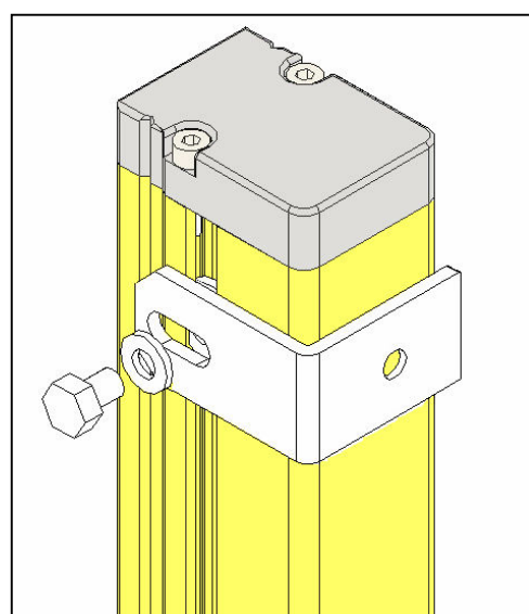
Brackets mounted on the barriers
