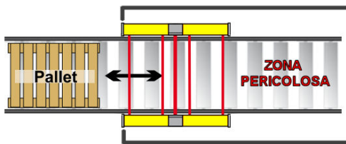
T model with parrallel beams( entry or exit )
