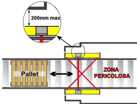
T model with across beams( entry or exit )
