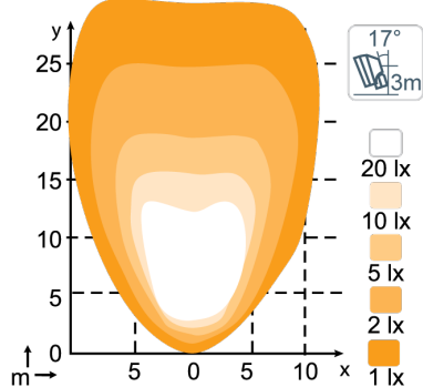
Scorpius PRO 5500, 5200lm Wide Flood
