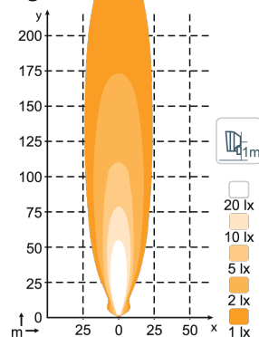
Scorpius PRO 5500, 5200lm High Beam
