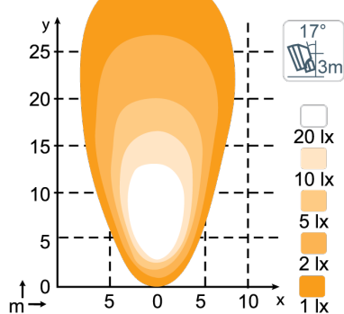
Scorpius PRO 5500, 5200lm Flood
