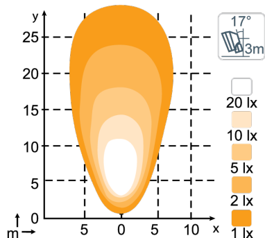
Scorpius PRO 3500, 3200lm Flood
