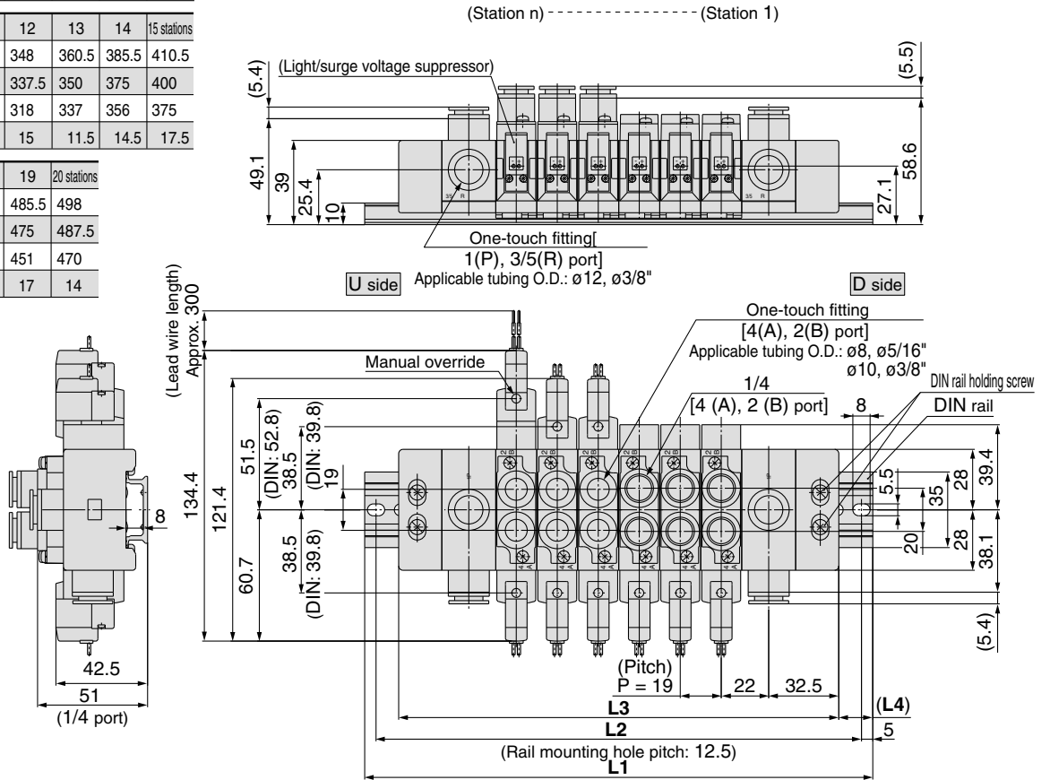
M plug connector (M)
