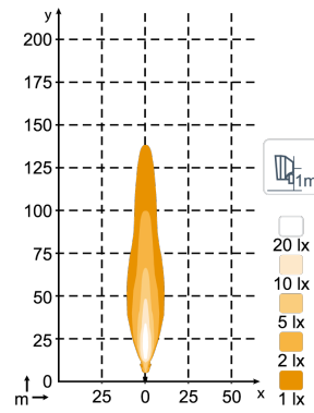
N5XX SAE High Beam
