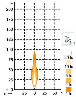
N5XX SAE Low Beam
